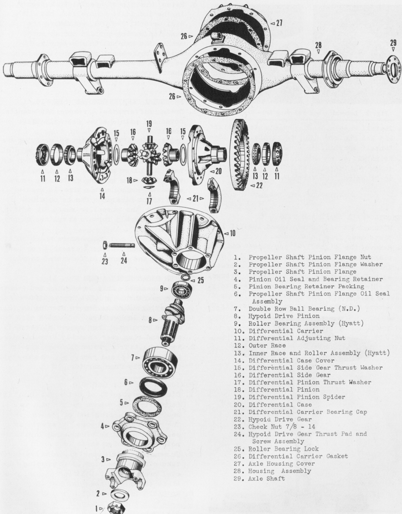
Fig. 1 Component Parts of Banjo Type Rear Axle
